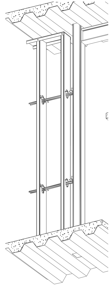
Assembly Detail
