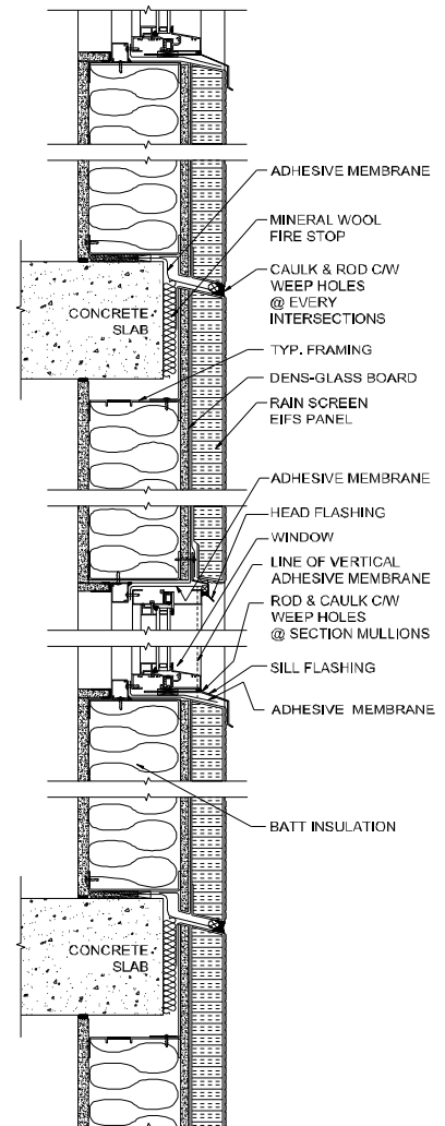
EIFS Wall Section
